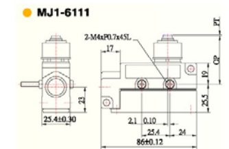
MJ1-6111 Enclosed limit switch, with seal boot, IP67
