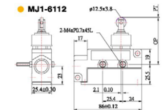
MJ1-6112 Enclosed limit switch, with seal boot, IP67
