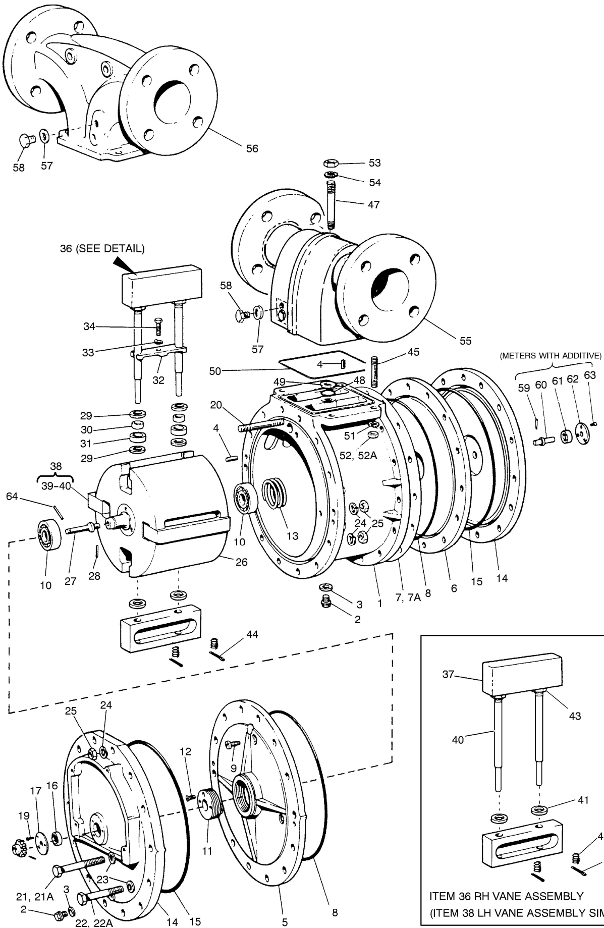
FIG 7.1 BULKMETER COMPONENTS
